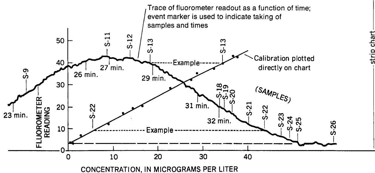
Figure 9.—Example of calibration of strip-chart trace. Selected samples from the fluorometer flow-through discharge are subsequently analyzed in the laboratory and concentrations are plotted against the strip-chart reading directly on the graph.
