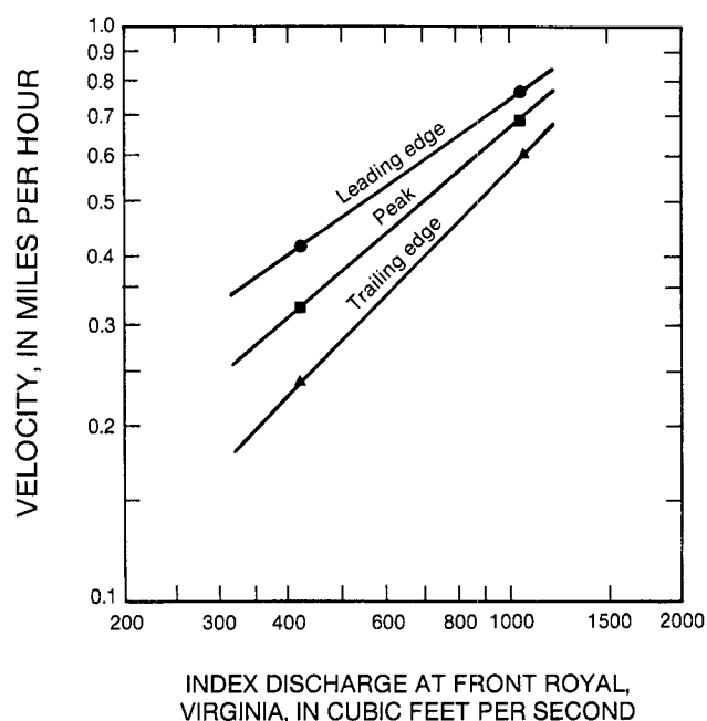
Figure 20.—Plot of traveltime velocities in reach between sites 7 and 8 as a function of index discharges at the Front Royal station on the South Fork Shenandoah River, Virginia (from Taylor and others, 1986).
