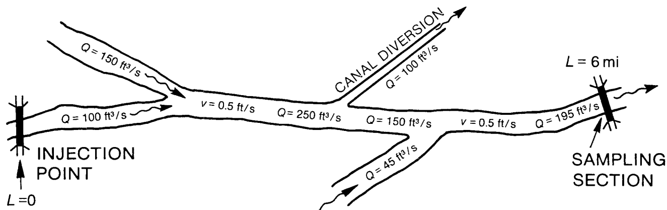
Figure 15.—Stream where flow is increasing in the downstream direction and a major diversion of flow occurs. (ft 3 /s, cubic feet per second; ft/s, foot per second; mi, miles; Q , stream discharge; v , velocity; L , stream length)
