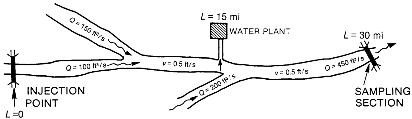
Figure 14.—Stream where a water user is involved and discharge is increasing in the downstream direction. (ft³/s, cubic feet per second; ft/s, foot per second; mi, miles; Q , stream discharge; v , velocity; L , stream length)
