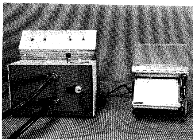
Figure 8.—Fluorometer equipped with a flow-through door and a strip-chart recorder for continuous sampling and recording.
